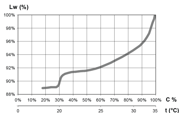
Graph 2 - Sound level Lw dB(A)
